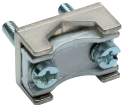
Borna racord cablu, 60mm 2 , NH00/60mm, 3 bucati
